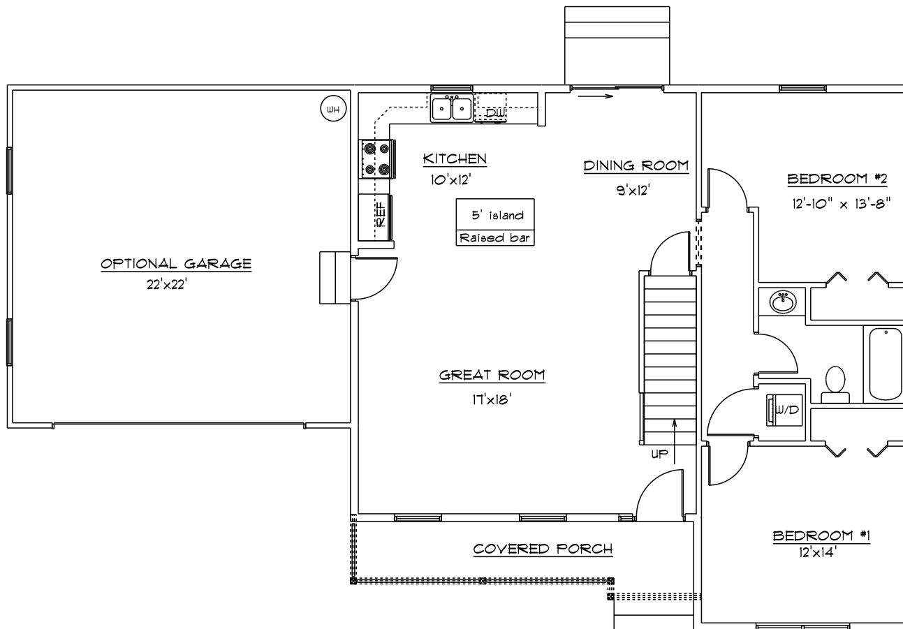
The Woodland First Floor Plan
