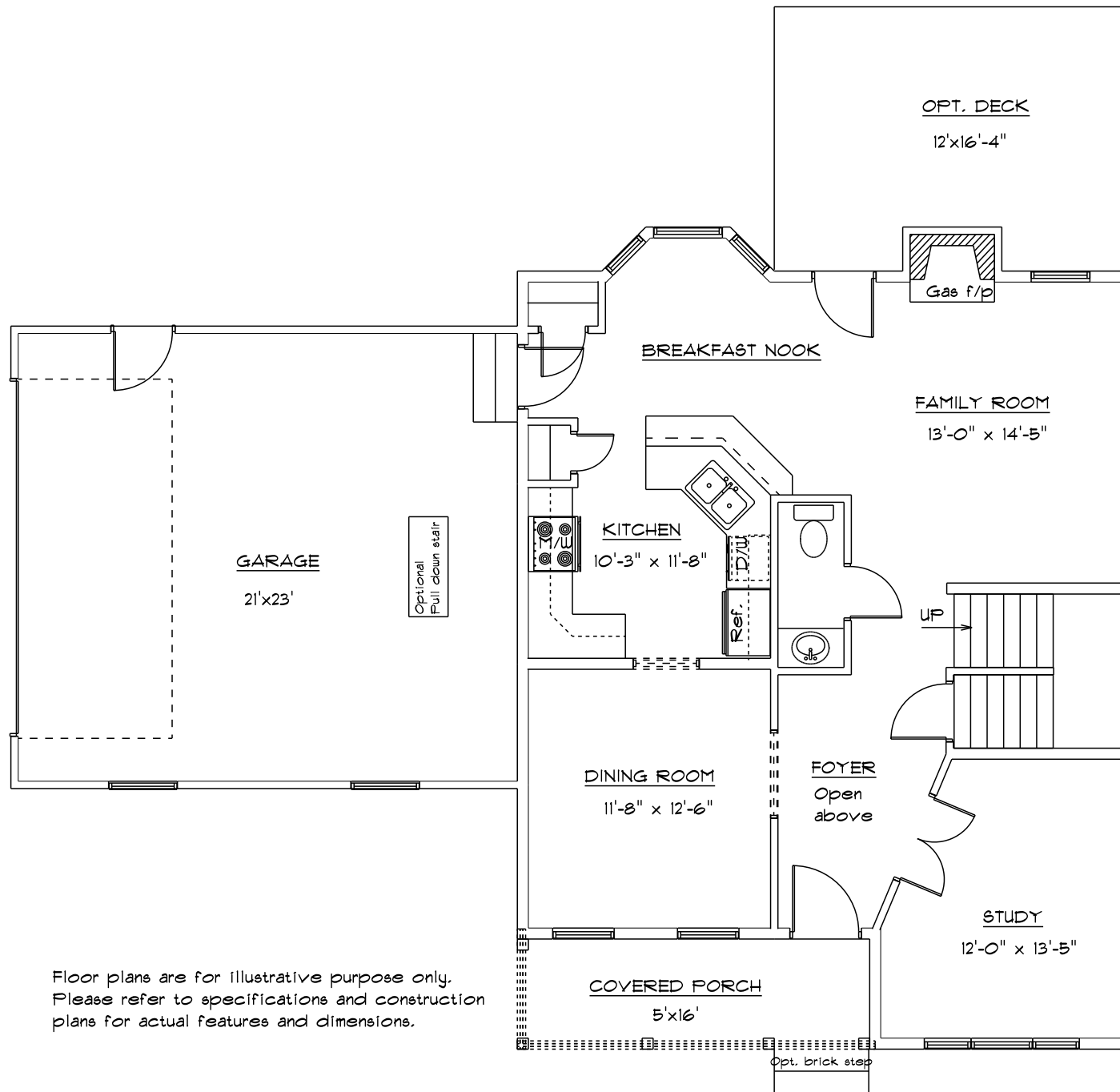
The Springhill First Floor Plan
