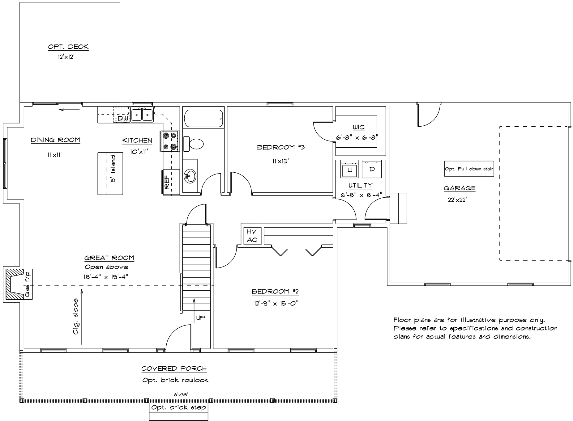
The Cape May First Floor Plan
